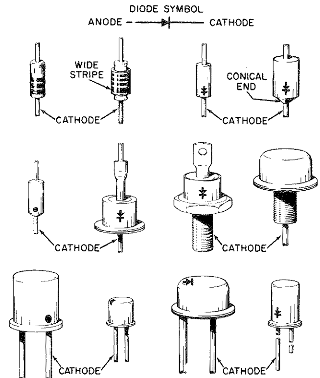
Figure 5-2. Examples of Diode Marking Methods
