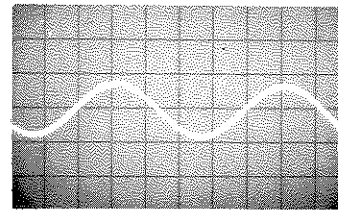
XA3 PIN 17 3.8MV P-P 40KC BANDWIDTH +2.6VDC
