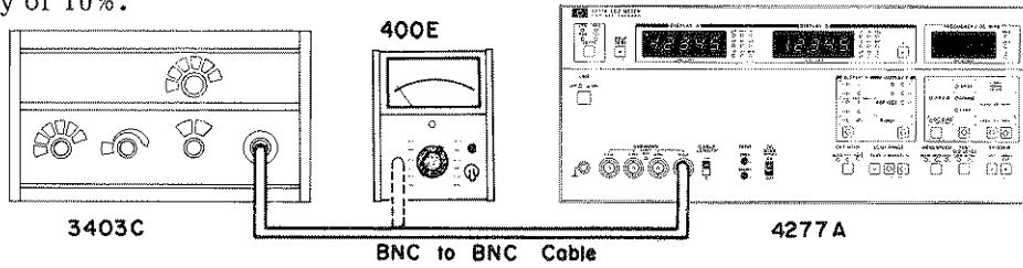
Figure 4-2. Test Signal Level Accuracy Test Setup.
