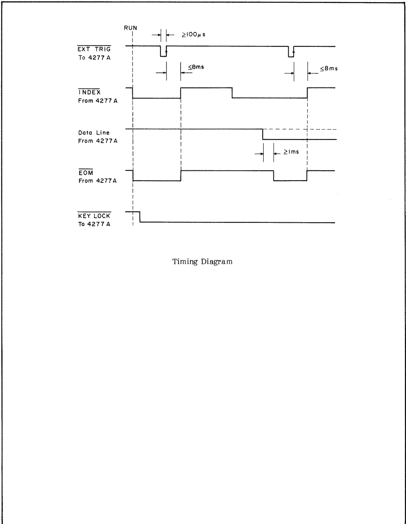
Figure 3-34. Option 002 Comparator (Sheet 7 of 7).
