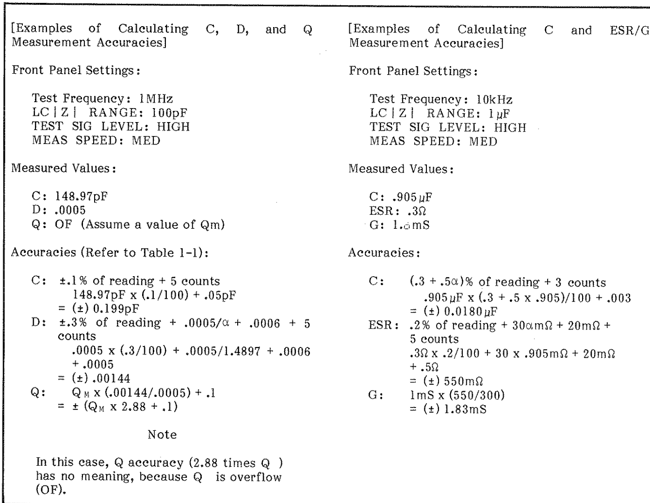
Figure 3-19. How to Calculate Measurement Accuracies.
