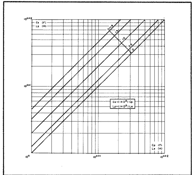
Figure 3-7. Parallel and Series Parameter Relationship.
