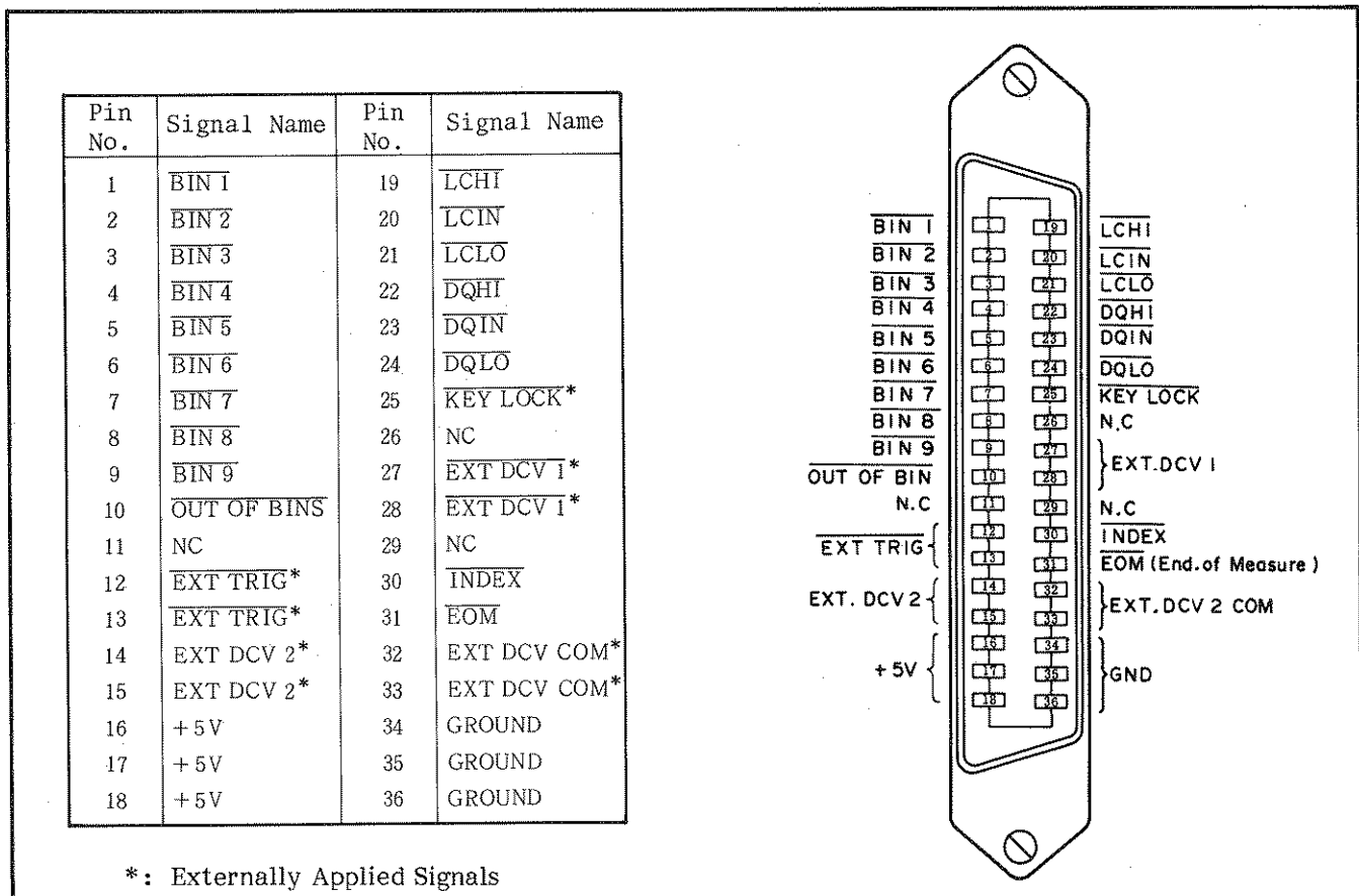
Figure 3-33. Pin Assignments for the Handler Interface Connector (HP 16064A).
