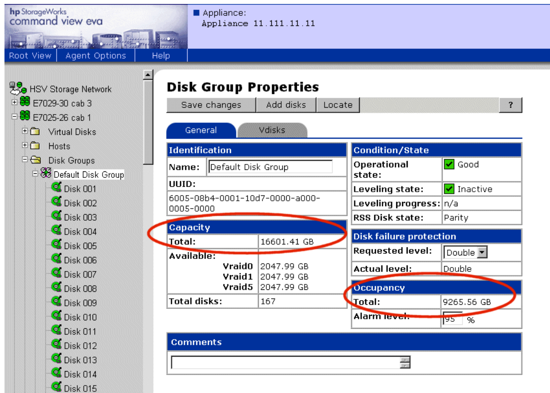
Figure 3.8. Command View EVA—Disk Group Properties page—checking free capacity
