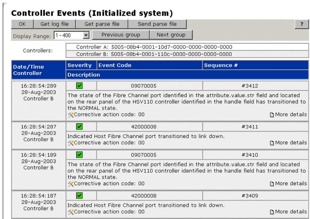
Figure 3.6. Command View EVA—Controller Events (Initialized system) page
