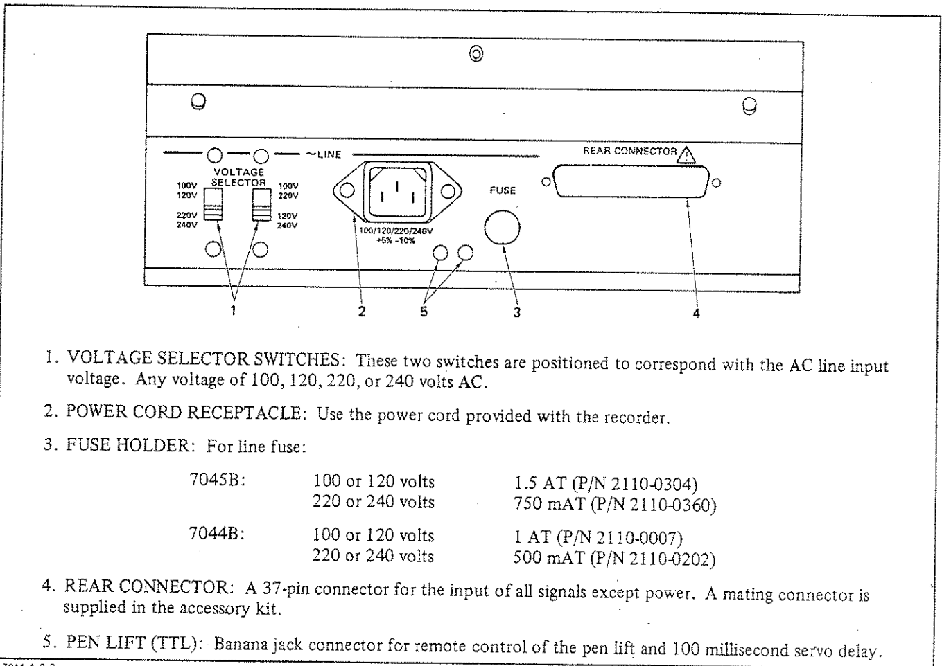
Figure 3-3. Rear Panel
