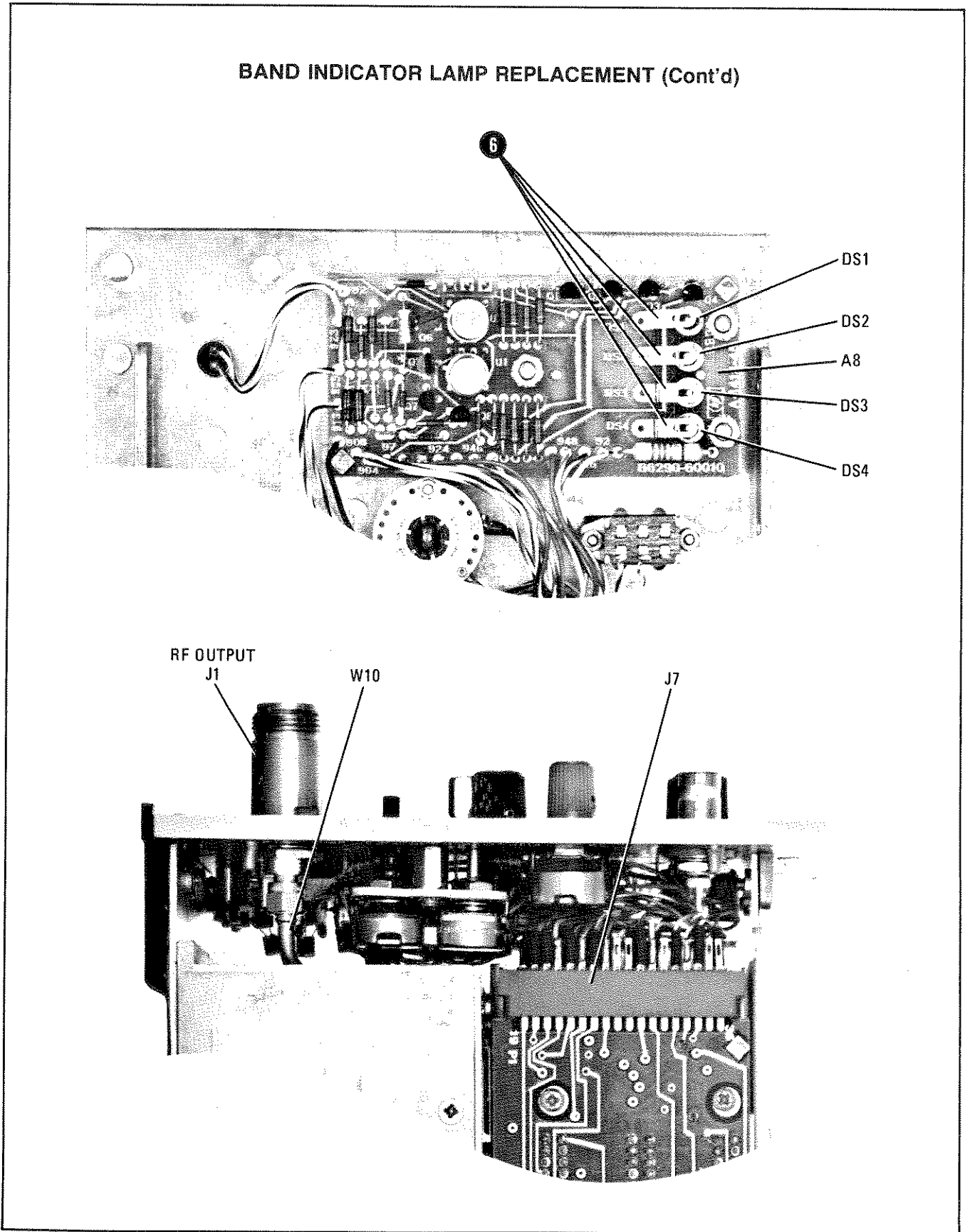
Figure 3-13. Band Indicator Lamp Replacement (2 of 2)
