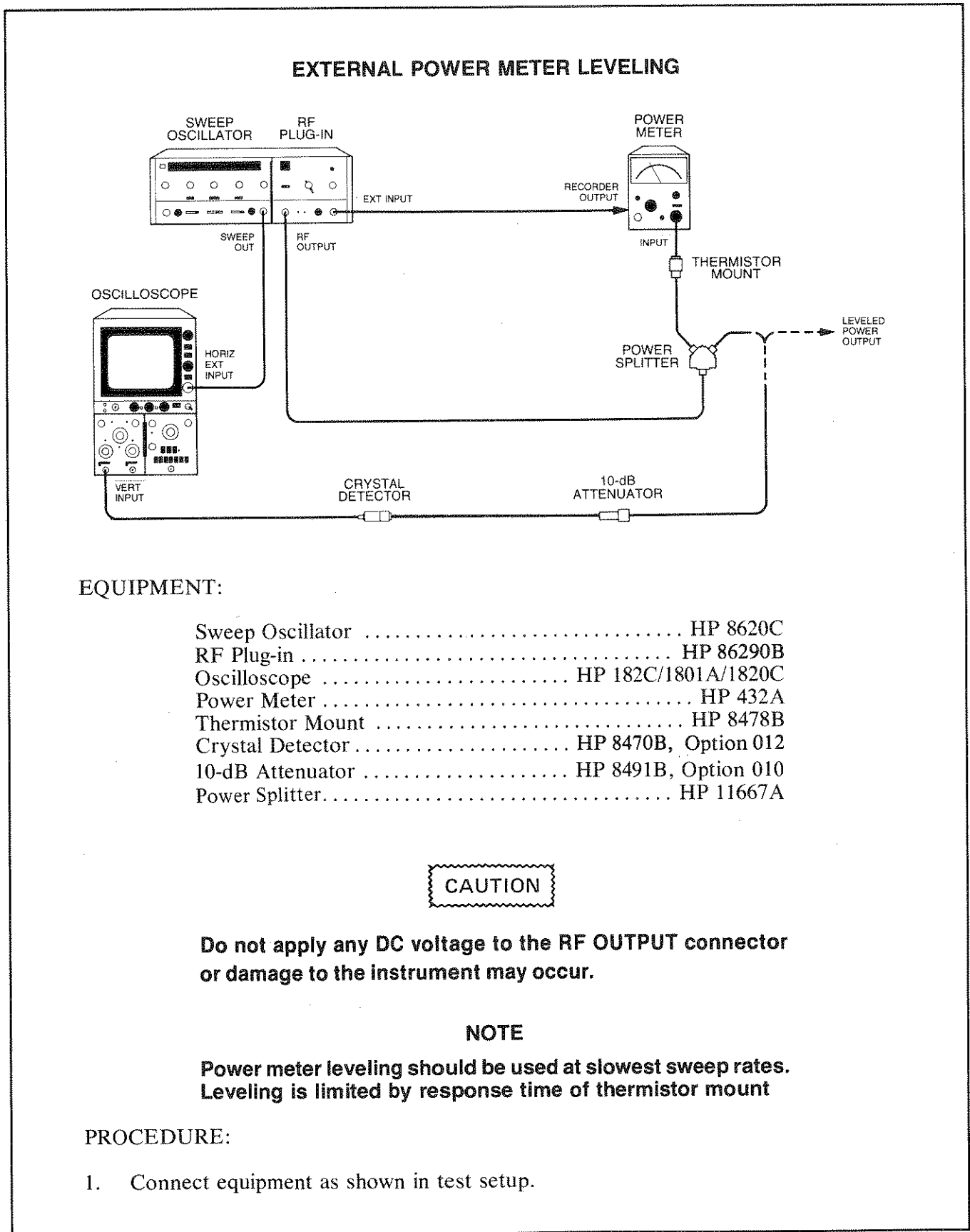
Figure 3-10. External Power Meter Leveling (1 of 2)
