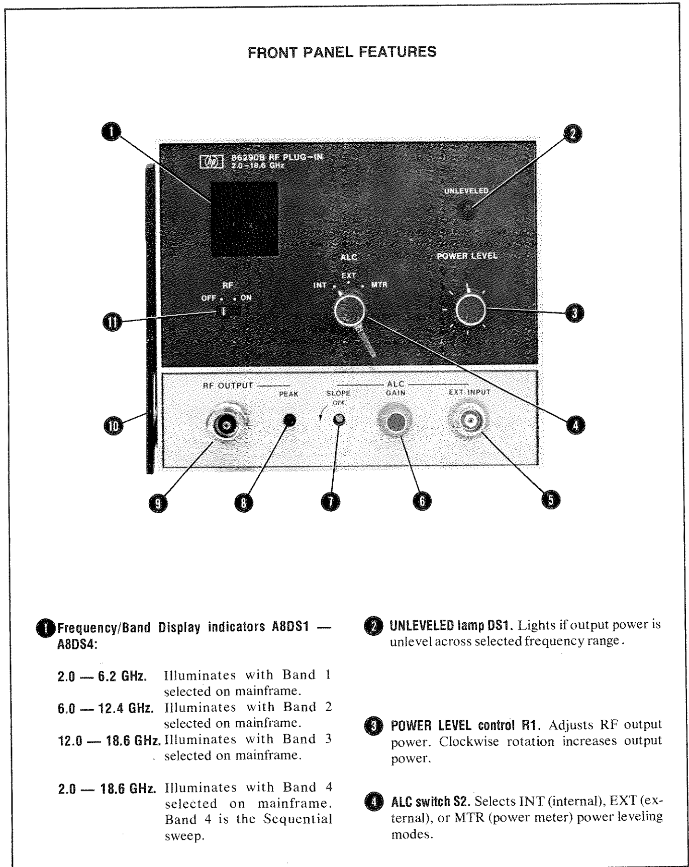
Figure 3-2. Front Panel Controls, Connectors and Indicators (1 of 4)
