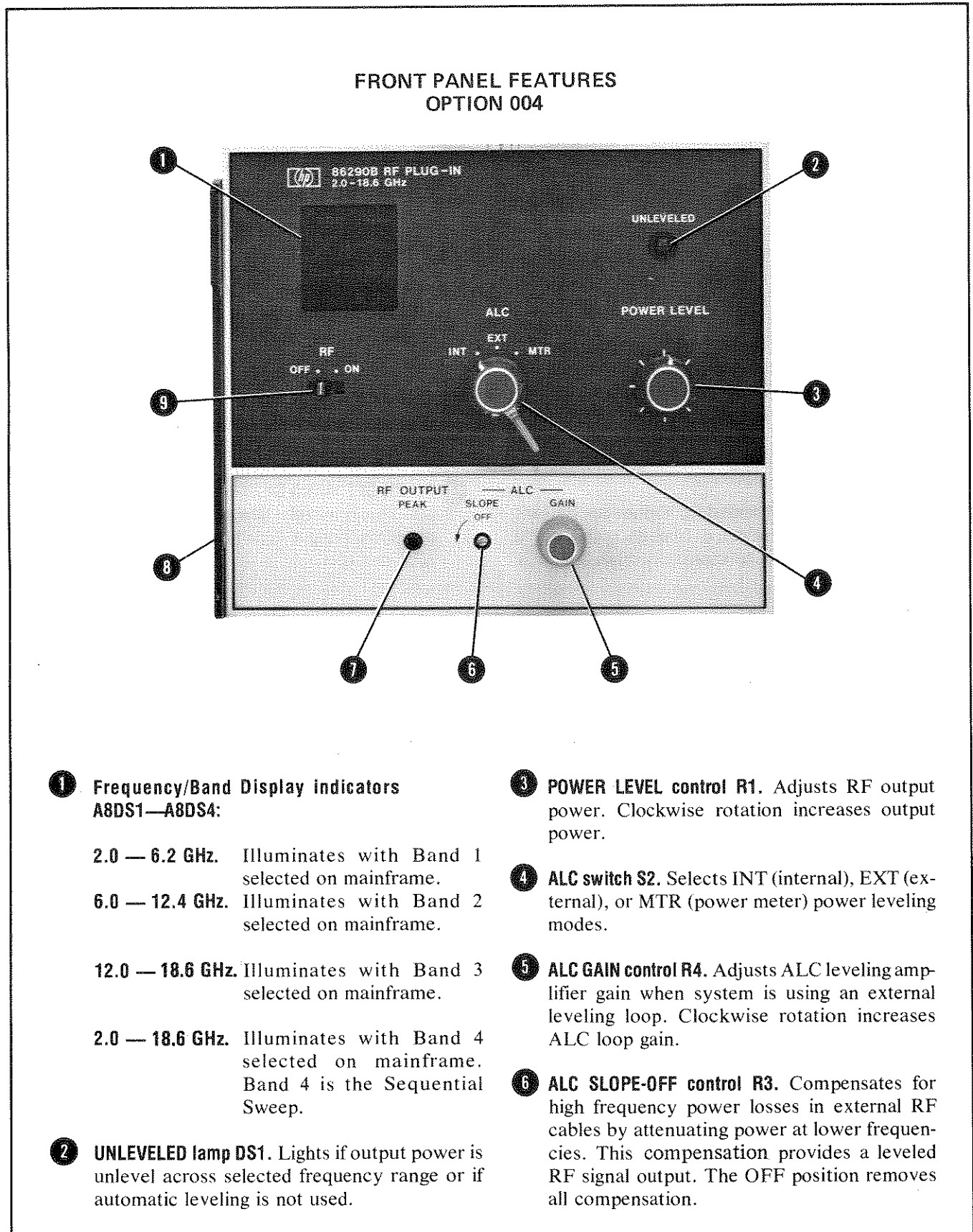
Figure 3-2. Front Panel Controls, Connectors and Indicators (3 of 4). Option 004
