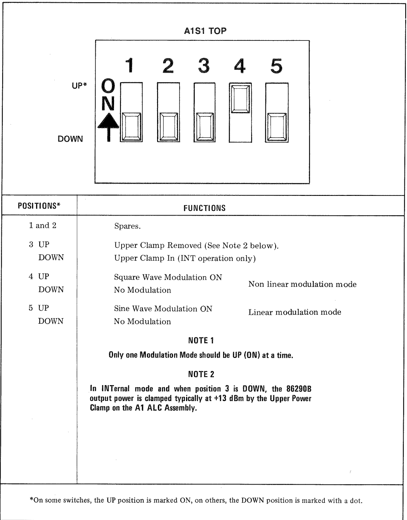
Figure 3-12. Switch Positions and Functions for ALC Function Switch AIS1
