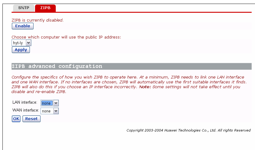
Figure 4-28 ZIPB setting
