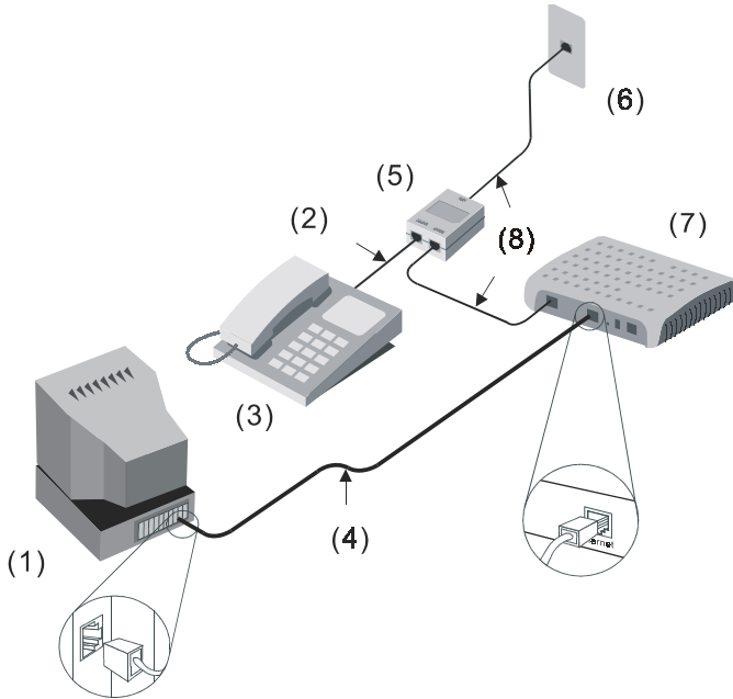
Figure 4 Computer to MT880 Connection
