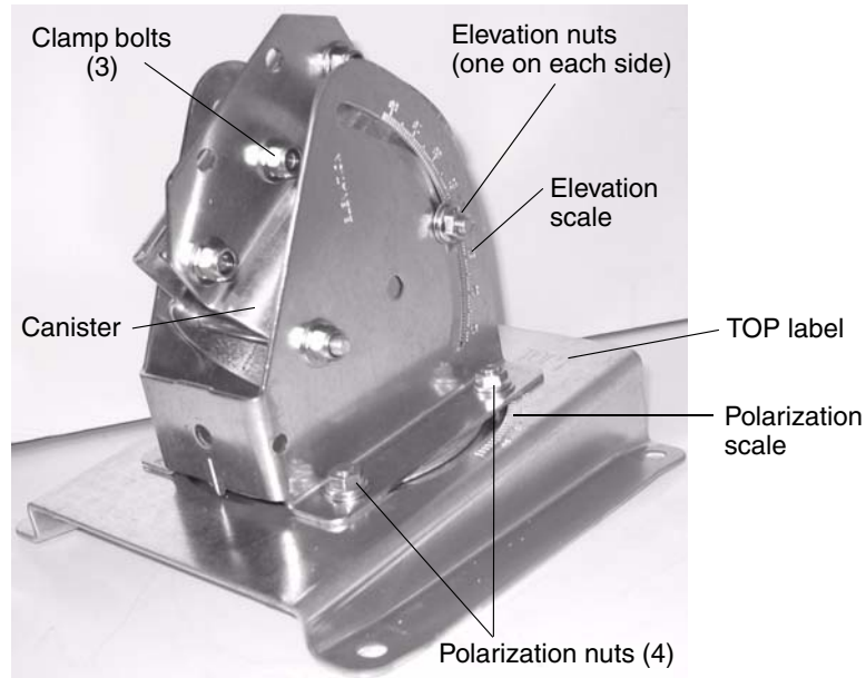
Figure 11: Antenna adjustments for elevation and polarization
