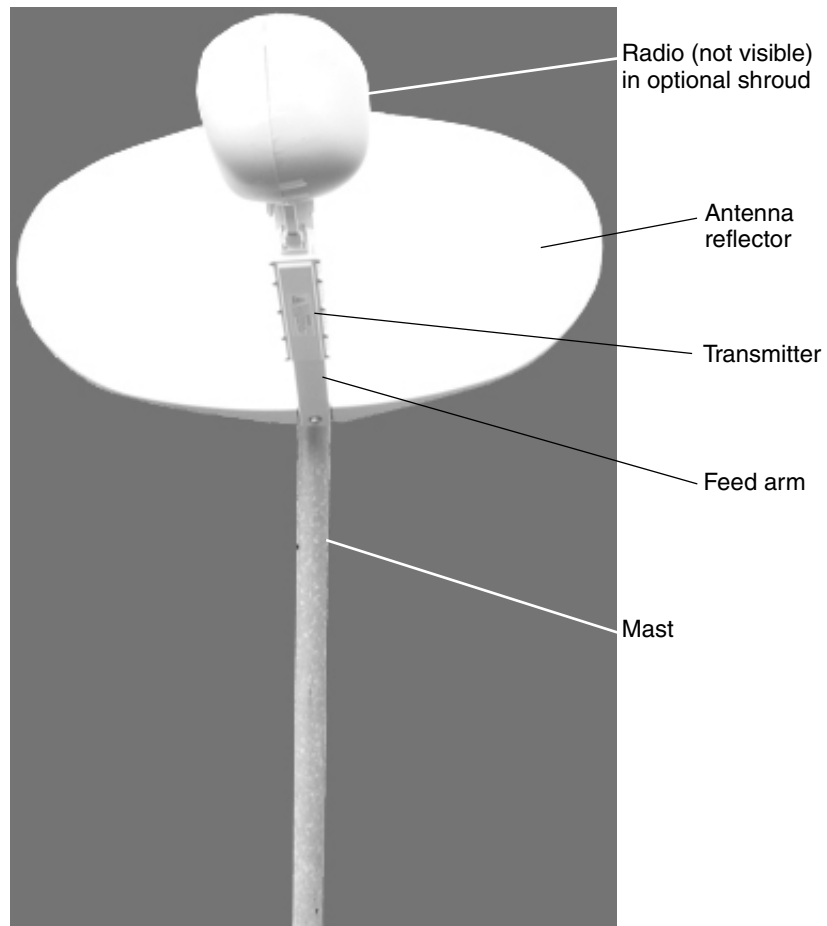
Figure 1: Installed .74 m antenna
