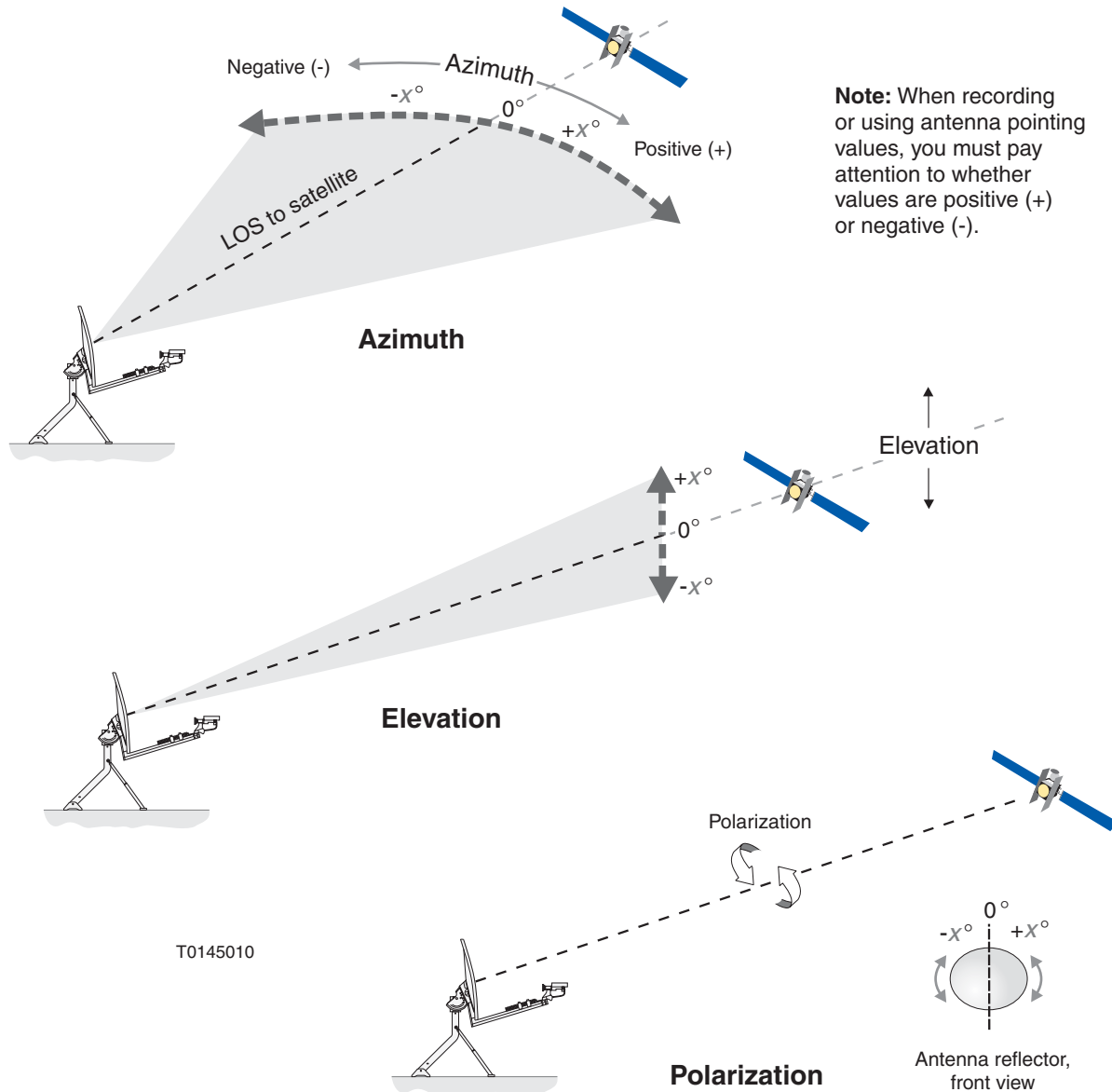
Figure 37: Adjusting azimuth, elevation, and polarization
