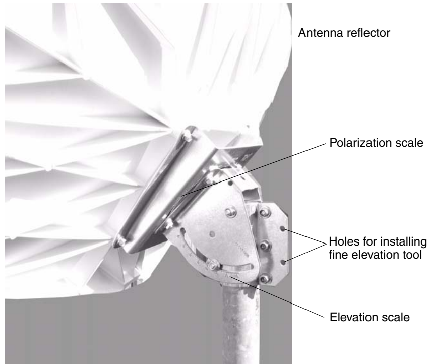
Figure 38: Pointing features on the Az/el cap
