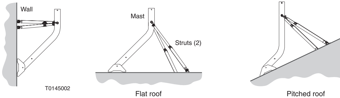
Figure 6: Trimast in various configurations
