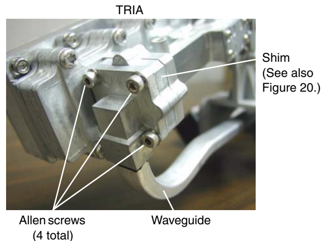
Figure 19: Shim location next to TRIA
