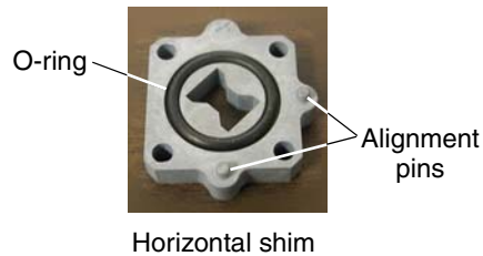
Figure 20: Horizontal shim and vertical shim for transmit polarization
