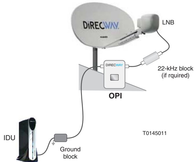
Figure 35: OPI
