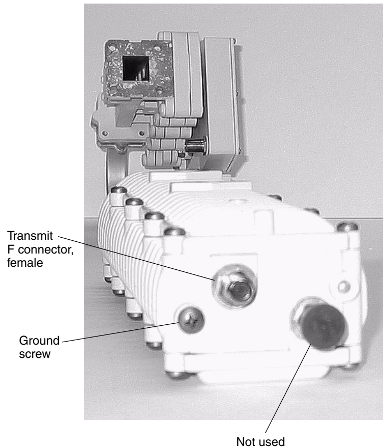
Figure 33: Ground screw on the transmitter
