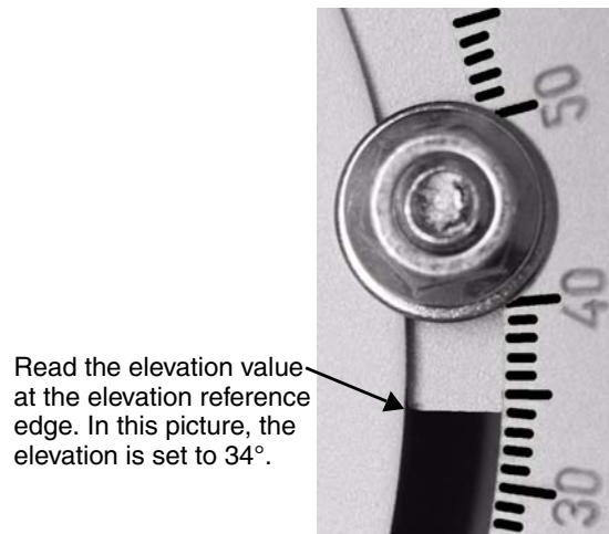
Figure 15: Reading the elevation reference edge
