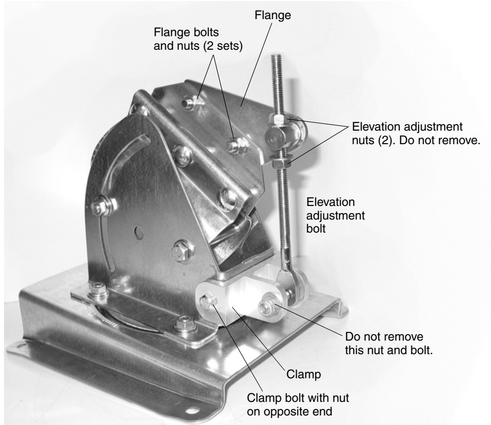
Figure 18: The fine elevation pointing tool
