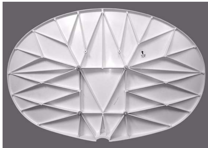
Figure 3: Antenna reflector (rear view)
