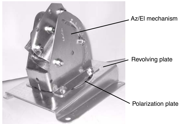
Figure 2: Az/el cap
