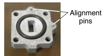
Vertical shim
