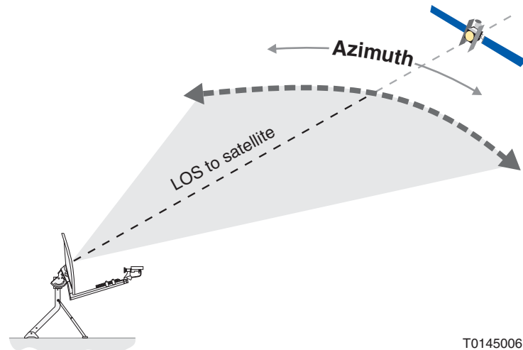
Figure 41: Adjusting azimuth
