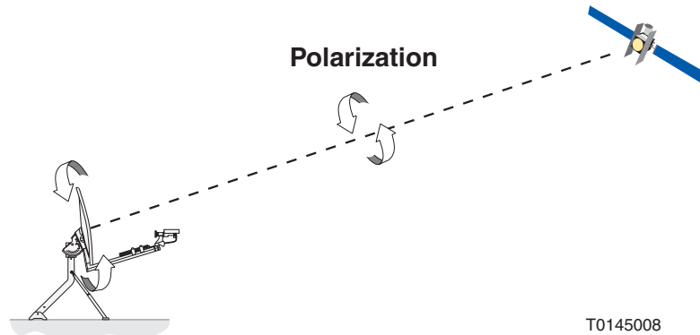
Figure 16: Adjusting polarization
