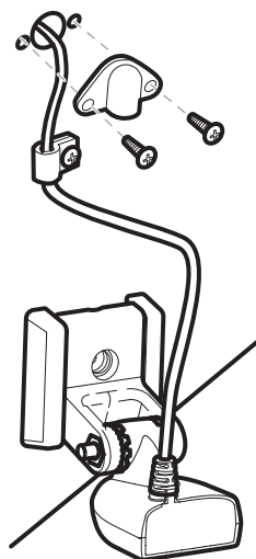
Routing the Cable
