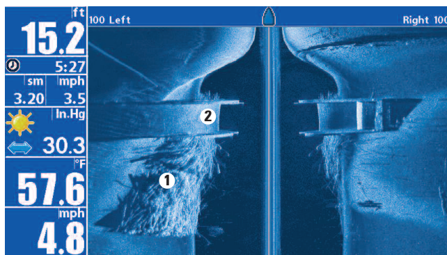
1 Dumped logs
