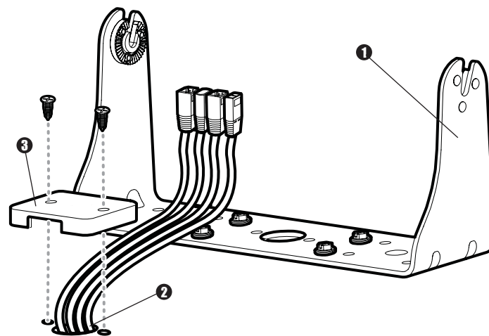
Cables Routed Behind Mounting Bracket
