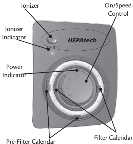
Figure 1 - Purifier Controls
