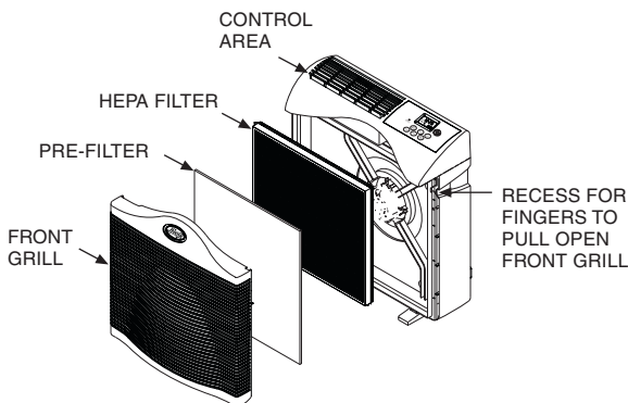
Fig. 2 - Air Purifier Components
