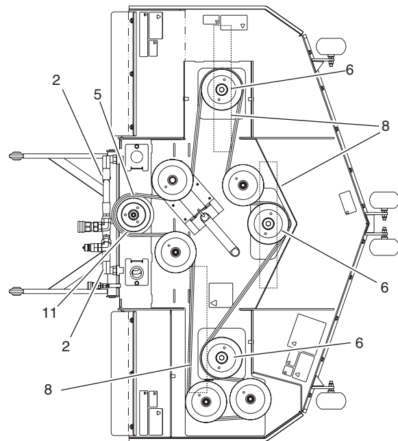
Rear discharge deck
